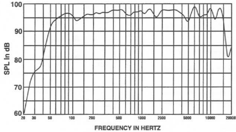
Figure 2—TS992-LX Typical Frequency Response with Presets of Dx34A Digital Speaker System Processor (swept sine-wave input, anechoic environment, 4 volts at 500 Hz at 10 feet, mic on an axis coincident with lower edge of the HF horn)
