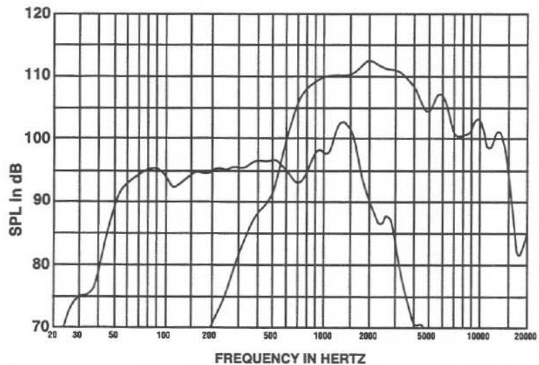
Figure 3—TS992-LX Typical Frequency Response of High- and Low-Frequency Sections Alone (swept sine-wave input, anechoic environment, 4 volts at 10 feet normalized for 1 watt at 1 meter, mic on an axis coincident with lower edge of the HF horn)
