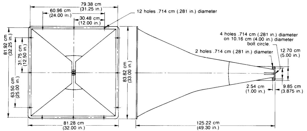
FIGURE 1 — Dimensions
