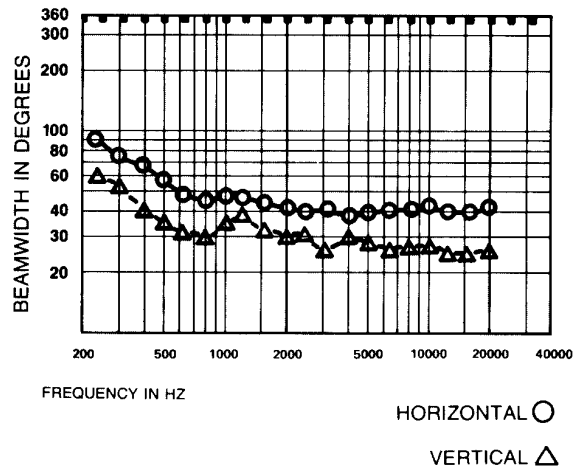
FIGURE 4 6-dB-Down Beamwidth versus Frequency
