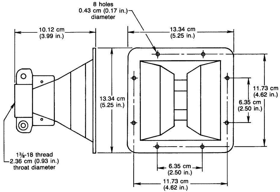
FIGURE 1 — Dimensions
