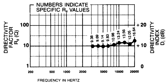
FIGURE 5 Directivity versus Frequency
