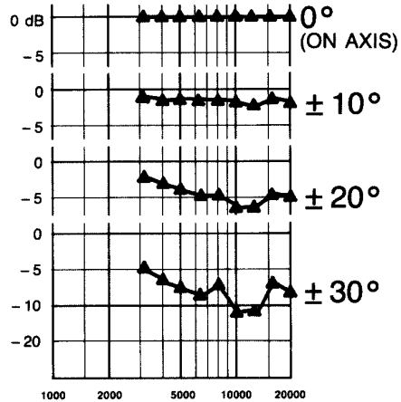
FIGURE 3 Vertical Off-Axis Response
