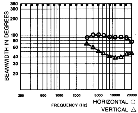
FIGURE 4 6-dB-Down Beamwidth versus Frequency
