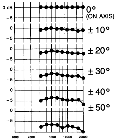
FIGURE 2 Horizontal Off-Axis Response
