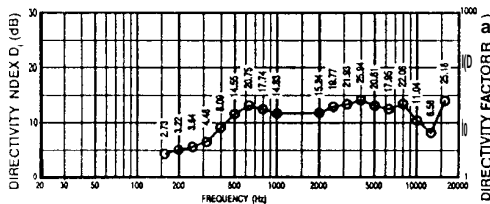
FIGURE 3 - Directivity Factor and Directivity Index vs. Frequency
