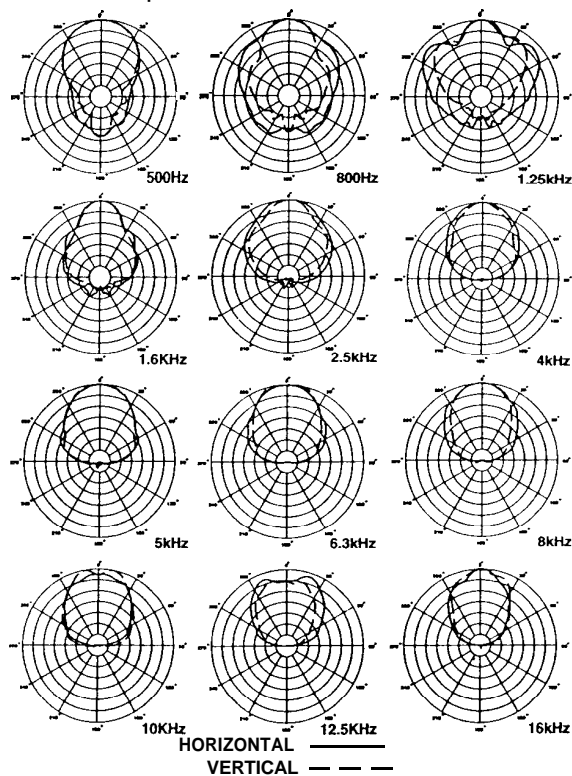
FIGURE 6 - Polar Response
